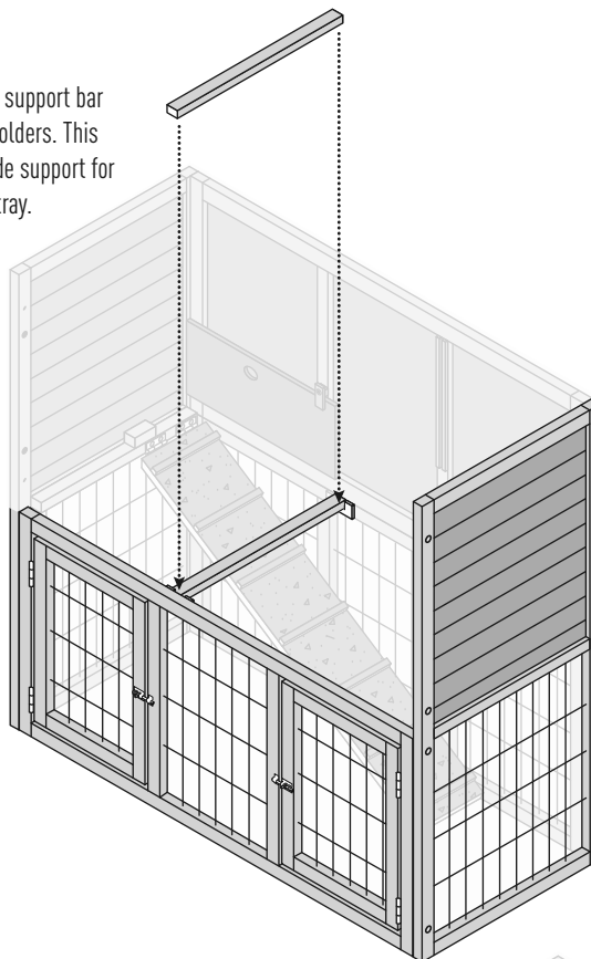
Cutaway view
